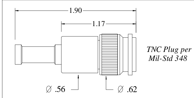
Features Not Shown : Safety Wire Holes, Gasket in Front
