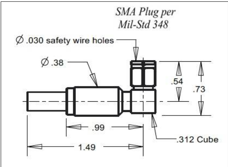
Features Not Shown : Safety Wire Holes, Gasket in Front
