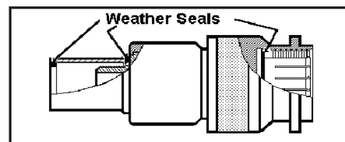
Figure 3. Typical connector weather-proofing. Shows recommended extra protection of dual-wall shrink tube over cable and connector. This covering might also be a wrapped sealant mentioned in the text below, and could cover the entire connection as well.
